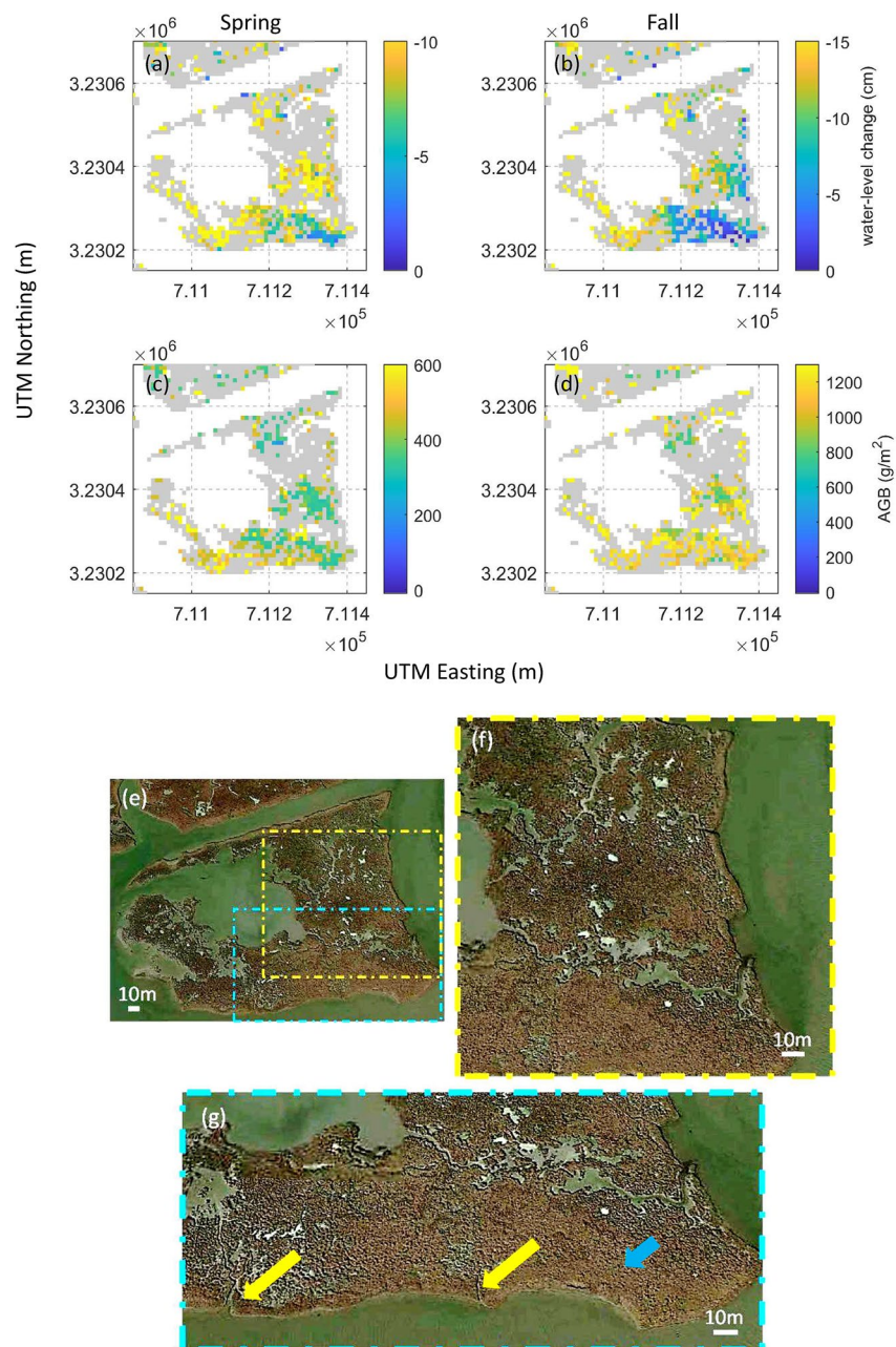
Figure 10. Spatial distribution of (a, b) UAVSAR-derived WLC (cm), and (c, d) AGB ( \text{g}/\text{m}^2 ) values in spring (a, c) and fall (b, d) for marsh 2. WLC was measured during the 12 April 2021 and 4 September 2021 Uninhabited Aerial Vehicle Synthetic Aperture Radar flights. Satellite images: (e) entire marsh 2; (f, g) close up of two different parts of the selected marsh. Images (f, g) highlight the presence of small tidal channels in the marsh landscape. The large (yellow) arrows highlight the presence of two small tidal channels with a width of 2–3 m. The small (blue) arrow indicates an area of the marsh where tidal channels are absent (image ©Google, Landsat/Copernicus).
